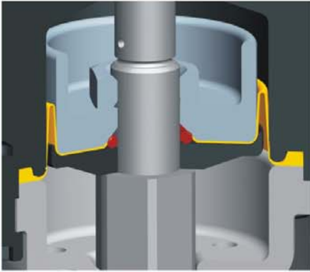
Sistema de balanceamento com diafragma rollout Balanced system with rollout diaphragm.
